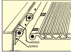
Figure 3 Bolt or welded hinge
